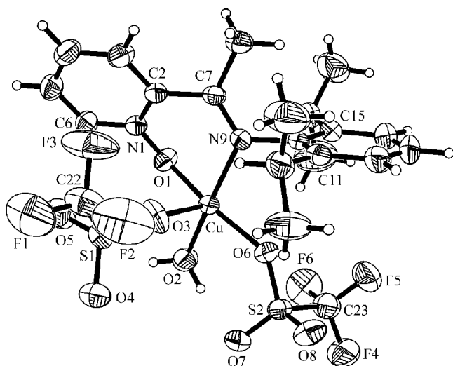
Figure 11. View of the molecular structure of complex 23a .
