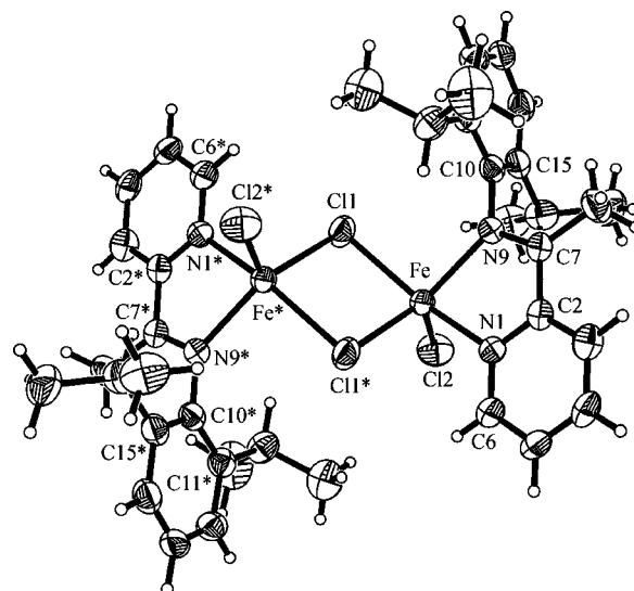
Figure 4. View of the molecular structure of the dimeric iron complex 15a .
