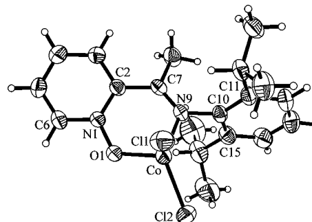
Figure 7. View of the molecular structure of the cobalt complex 20a .
