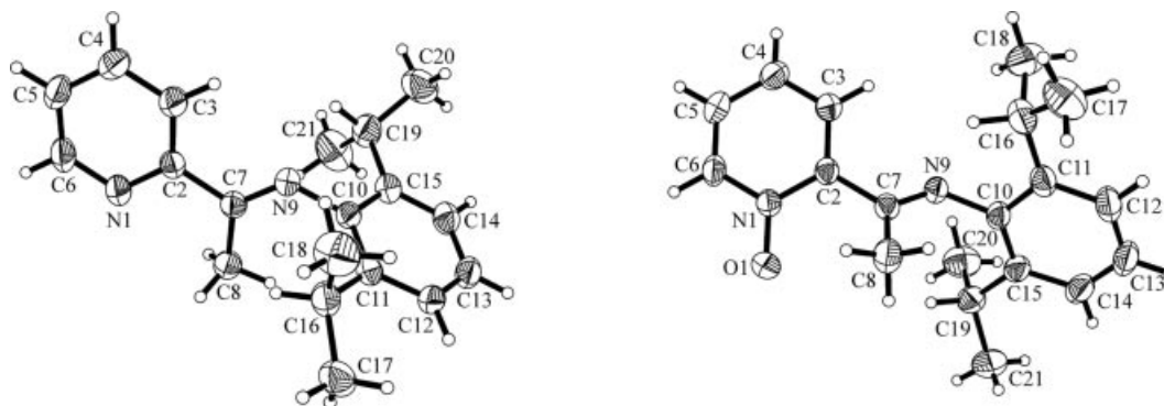
Figure 1. Comparison of the molecular structures of the ligand systems 3a (left) and 2a (right).
