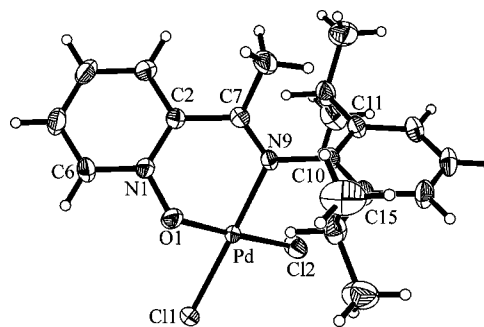
Figure 6. Molecular structure of palladium complex 19a .
