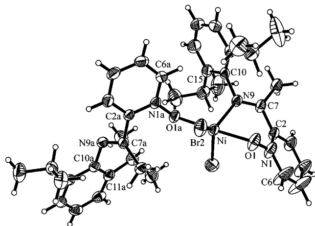
Figure 9. View of the molecular structure of complex 21a .
