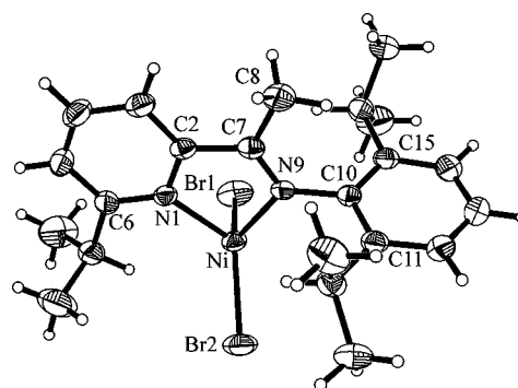
Figure 3. Molecular structure of the nickel chelate complex 14b .
