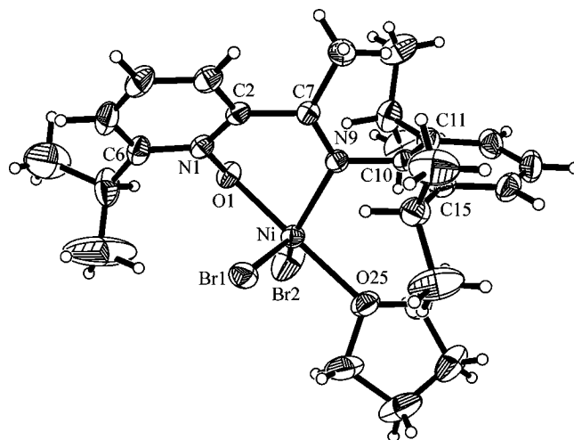
Figure 8. Molecular geometry of the nickel(II) complex 21b .
