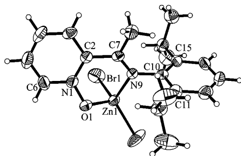
Figure 10. View of the molecular structure of complex 22a .
