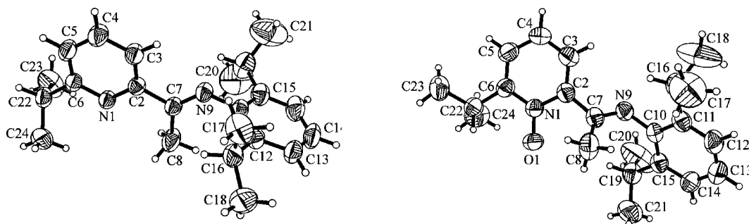
Figure 2. Comparison of the conformational arrangements of the chelating ligand systems 3b (left) and 2b (right).
