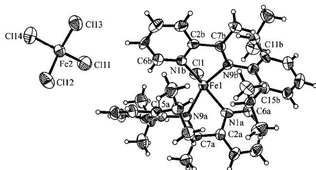
Figure 5. Molecular structure of the salt [(3a) 2 FeCl] + [FeCl 4 ] − ( 18a ).
